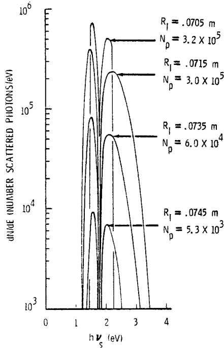
Fig. 6. Plot of dN/dE vs. h\nu_s for Gaussian distribution in \mu centered about \mu_0 = 0 with \Delta\mu = 0.1 .
