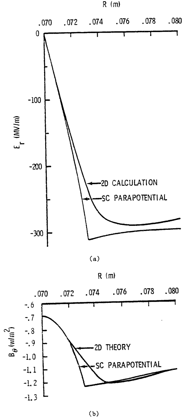
Fig. 2. Plot of \bar{E} and \bar{B} fields extrapolated from data points of Bergeron and Pqukey 2 and according to SC parapotential 3 theory.
