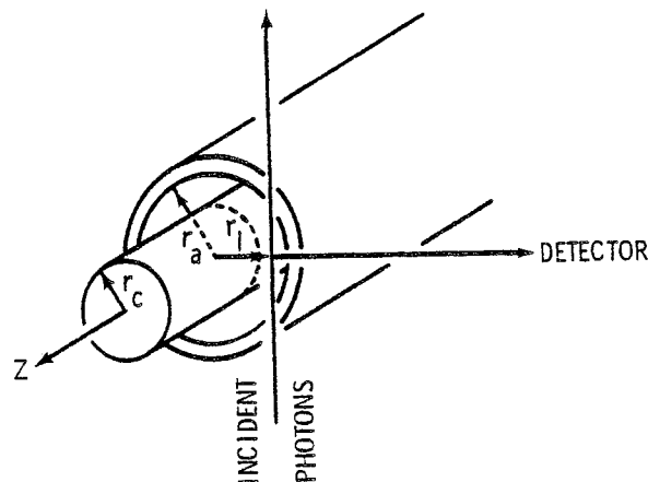
Fig. 1. Coax with basic features of Compton scattering experiment. Directions of electron power flow (+Z), incident photons, and detector are all mutually perpendicular.
