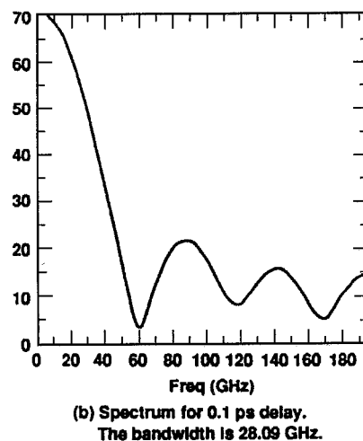
Figure 7. Voltage spectra generated by wave interference.
