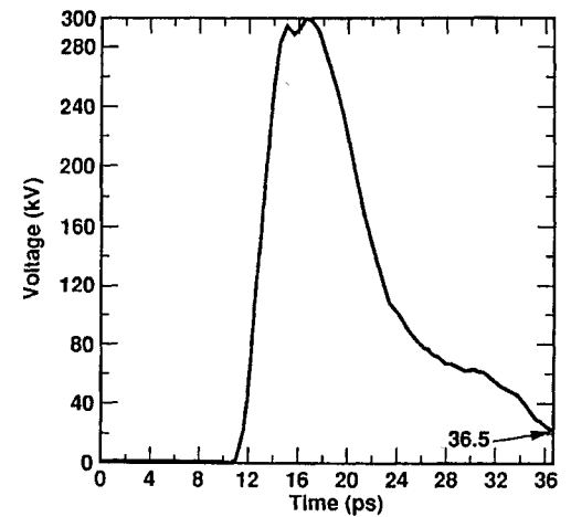
Figure 4a. Voltage waveform at right boundary at 292.4 kV and 27.2 atm.
