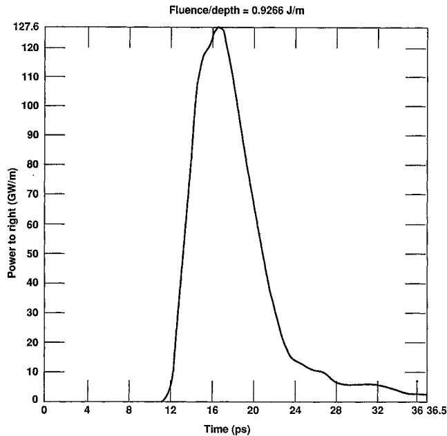
Figure 5a. Instantaneous power across right boundary.
