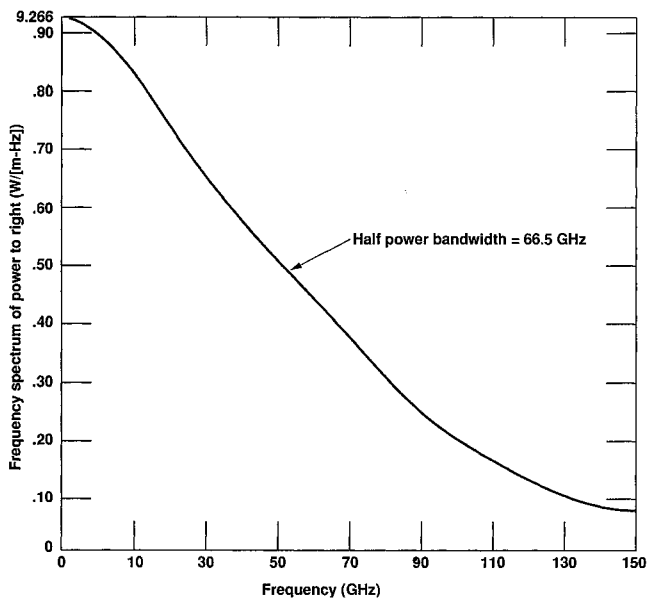
Figure 5b. Frequency spectrum of the instantaneous power across right boundary.
