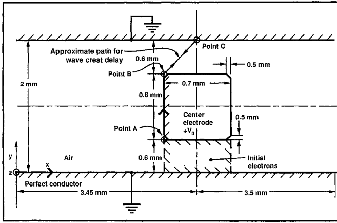
Figure 1. The pulse generator switch model.
