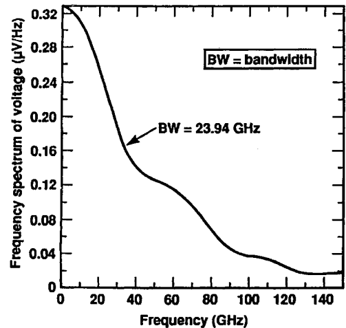
Figure 4b. Frequency spectrum of the voltage at 292.4 kV and 27.2 atm.
