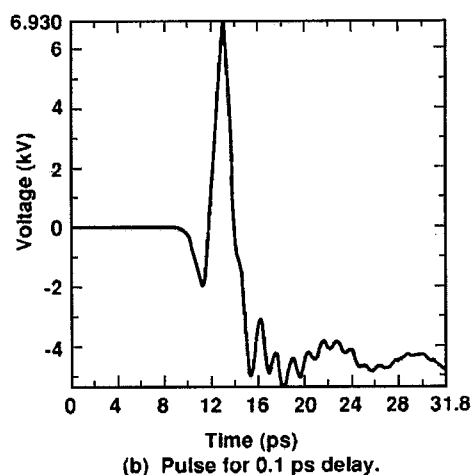
Figure 6. Voltage waveforms generated by wave interference.
