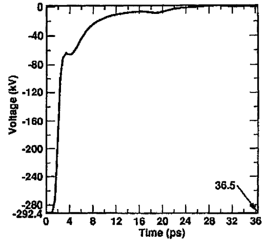
Figure 3. Waveform of the voltage between the center electrode and the bottom plate near the vertical center line.
