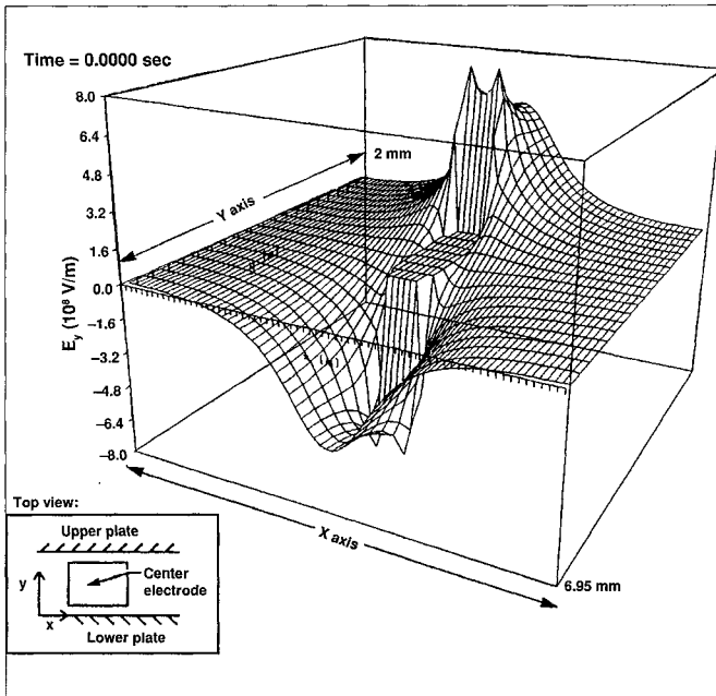
Figure 2. Initial distribution of E_y .
