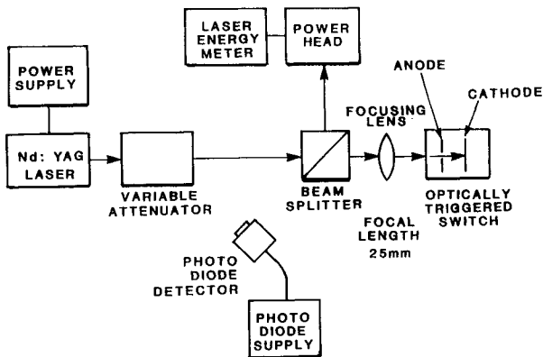
Fig. 3. Experimental optical setup.
