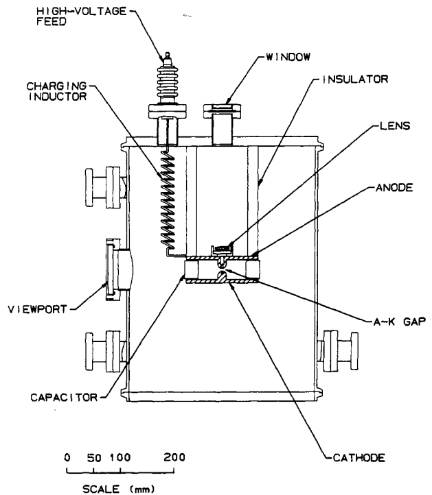
Fig. 1. Laser-triggered switch.
