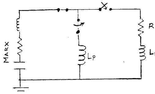
Figure 3. Schematic of Simulation Circuit.
