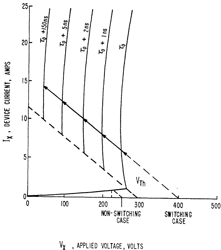
Figure 2. Post-switching MOTS currents as function of applied voltage and of time.
