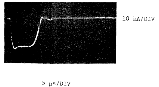
Figure 6. Load Current at E_{py} = 25 kV for Compact Megawatt Modulator with CX 1536A Thyatron
