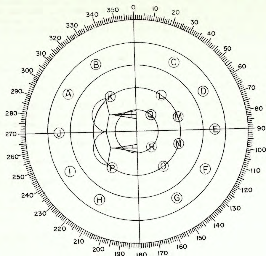
Fig. 1. PPI overlay showing location of GRP and approach and landing facilities in the approach control zone. The lettered circles represent ground reference points (GRP). The pattern-feeder controller could designate a flight path by giving the GRP's as destinations. The pilots could then direct their aircraft to the GRP's by using the API.
