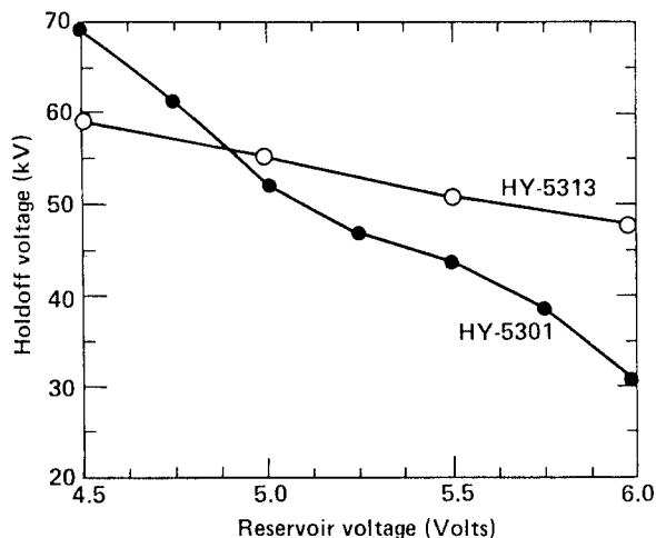
Fig. 3 Variation of holdoff voltage with reservoir voltage
