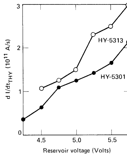
Fig. 4 Reservoir voltage dependence of di/dt at 200 Hz and 38 kV
