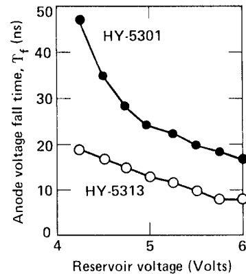
Fig. 5 Anode voltage fall time vs. reservoir voltage measured in a high inductance discharge circuit
