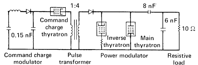
Fig. 1 Simplified circuit diagram of MCTF system.
