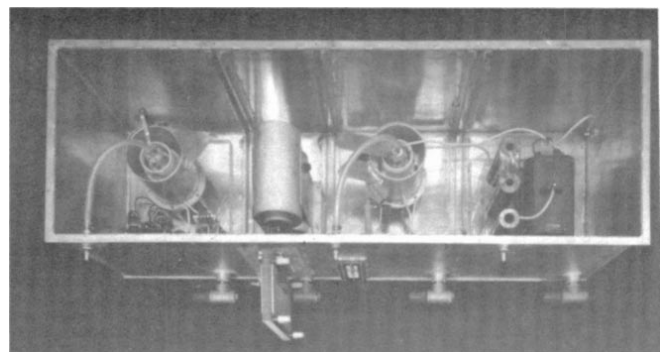
Fig. 2 MCTF modulator tank.
