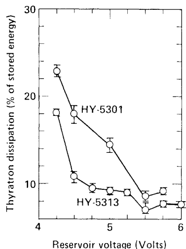
Fig. 6 Percent of thyatron dissipation as a function of reservoir voltage at 200 Hz and 38 kV
