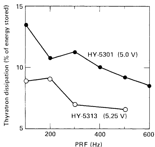
Fig. 7 PRF dependence of percent of thyatron dissipation. HY-5301 at 5.0 volts on reservoir HY-5313 at 5.25 volts on reservoir 38 kV charge voltage
