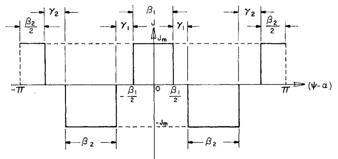
Fig. 2. Developed view of compulsator winding current sheets
