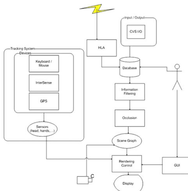
Fig. 6 Software structure of the AR system
