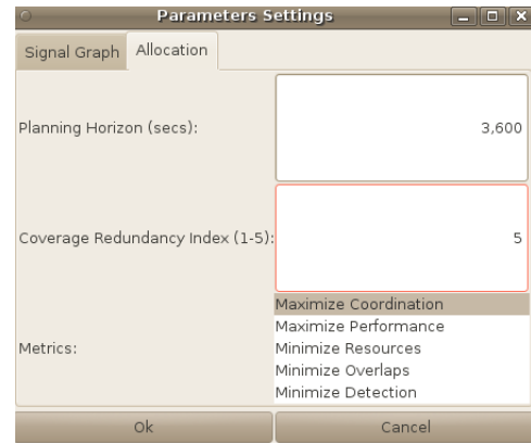
Figure 4. Interface for optimization settings in SAT. The coverage redundancy index indicates whether a penalty should incur due to overlaps in target coverage.
