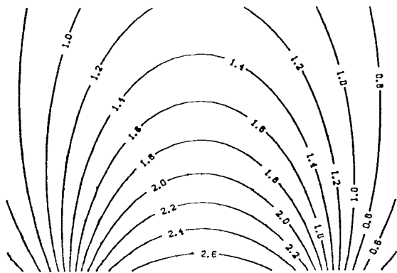
Figure 1. Example of electric field solution in rectangular coordinates.
