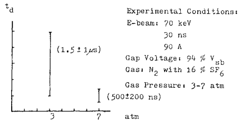
Fig. 8 f. Delay Time vs Gas Pressure.
