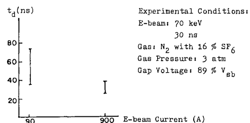
Fig. 7b. Delay Time vs E-beam Current.
