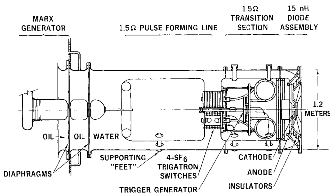
Figure 2. BLACKJACK 2, 1.5 \Omega electron beam accelerator. Output power, 0.6 TW.
