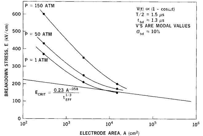
Figure 3. Variation of water breakdown stress with pressure and area.
