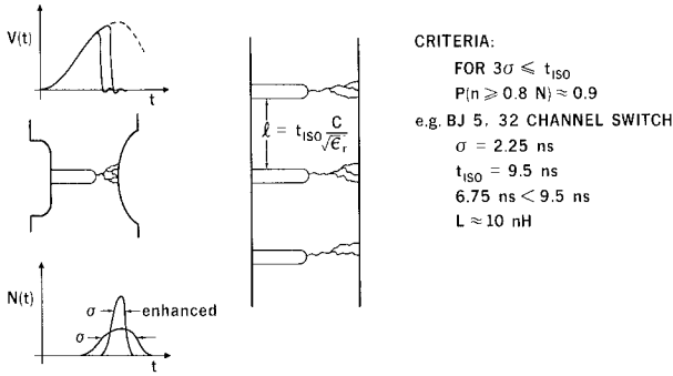
Figure 4. A rationale for multisite, multichannel water switches.
