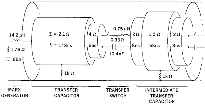
Figure 11. Part of BLACKJACK 5 pulseline model.
