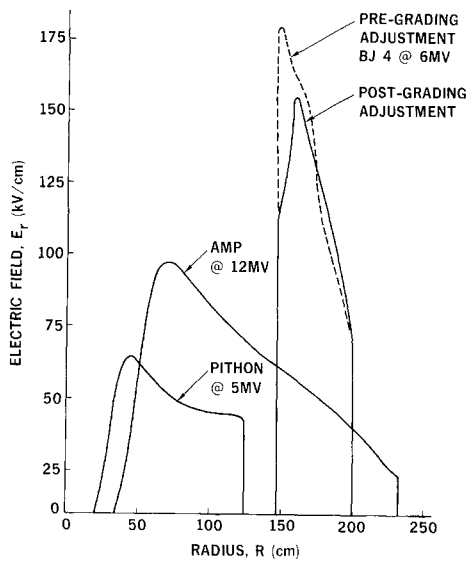
Figure 9. Pulseline diaphragm stress for BLACKJACK 4 and BLACKJACK 5 transfer capacitor, (AMP and Pithon diaphragm stresses included for comparison).
