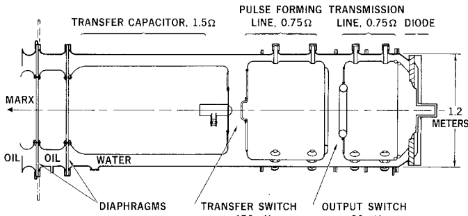
Figure 5. 3/4 \Omega , 1.3 TW BLACKJACK 3 pulseline cross section.
