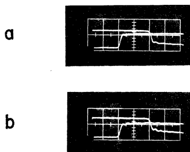
Fig. 8. Oscillograms showing leading and falling edges of probe input voltage (a) and output voltage (b) at sweep speeds of 2 ns/div.
