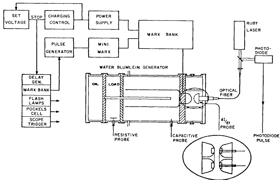
Fig. 1 Experimental Arrangement
