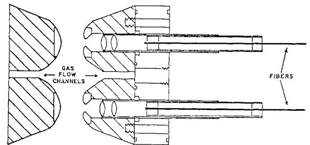
Fig. 3 Output Optics and Electrodes
