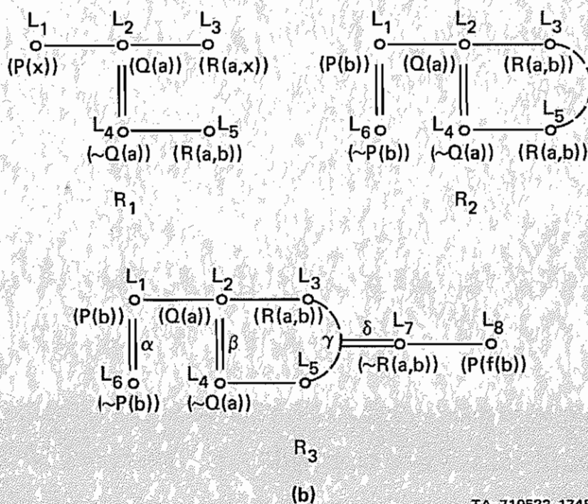
FIGURE 2 SUBSTITUTIONS DETERMINED BY GRAPH STRUCTURE
