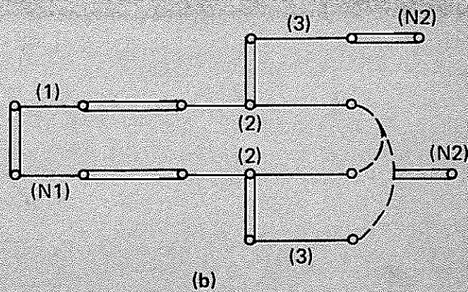
FIGURE 13 PROOF WITH POOR CHOICE OF STARTING CLAUSE
