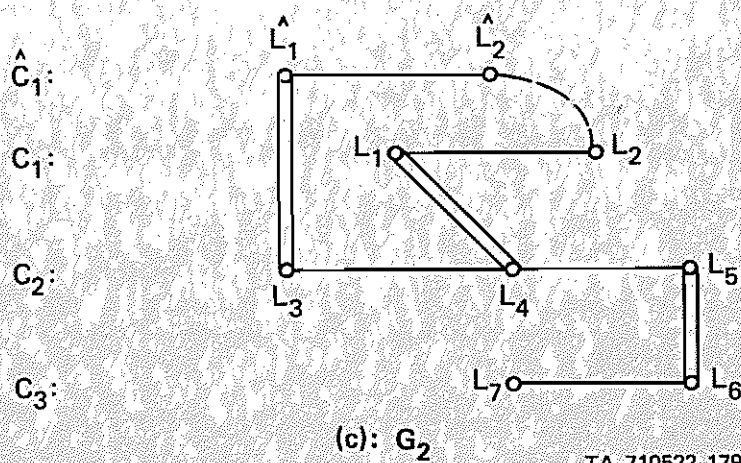
FIGURE 5 GRAPH DOMINANCE
