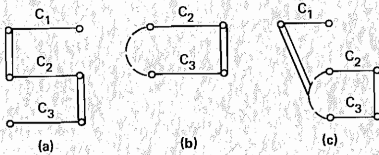
FIGURE 6 EXAMPLE OF ORDER DEPENDENCE
