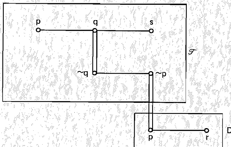
FIGURE 7 GRAPH WITH A TAUTOLOGICAL SUBGRAPH
