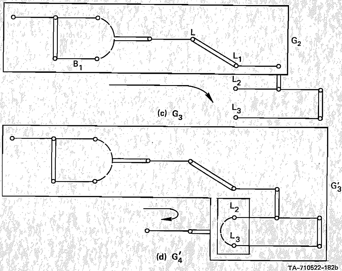
FIGURE 10 CONSTRUCTION OF A DEDUCTION SATISFYING THE CONSTRAINTS OF THEOREM 2 Continued
