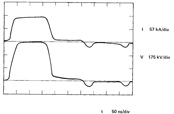
Fig. 8 Output pulse - resistive load
