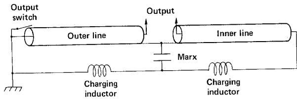
Fig. 3. Charging circuit
