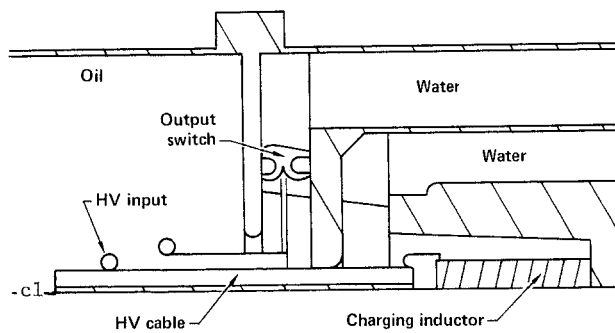
Fig. 4 Output switch configuration
