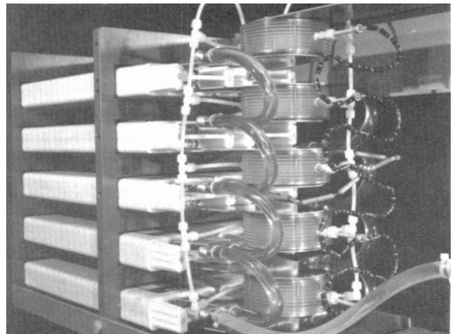
Fig. 2. 'B' amplifier Marx generator
