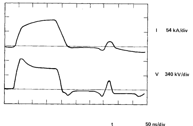
Fig. 9 Output pulse - diode load
