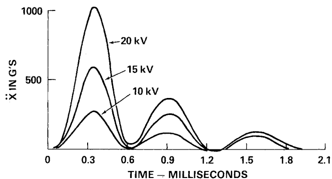
FIGURE 3 PREDICTED SHOCK PROFILES FOR EDESS-1
