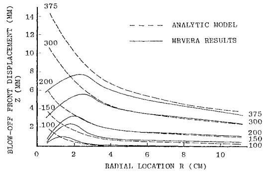
Figure 5. Blow-off front along 2 cm gap BJ3 disk diode.
