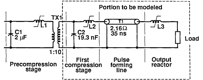
Figure 1. Simplified circuit diagram of the MAG-1-D magnetic pulse compressor.
