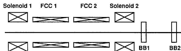
Fig. 6. Fast correction coil beamline layout.
