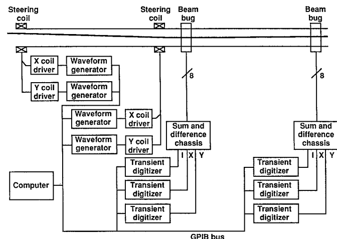
Fig. 7. Fast correction coil controls block diagram.
