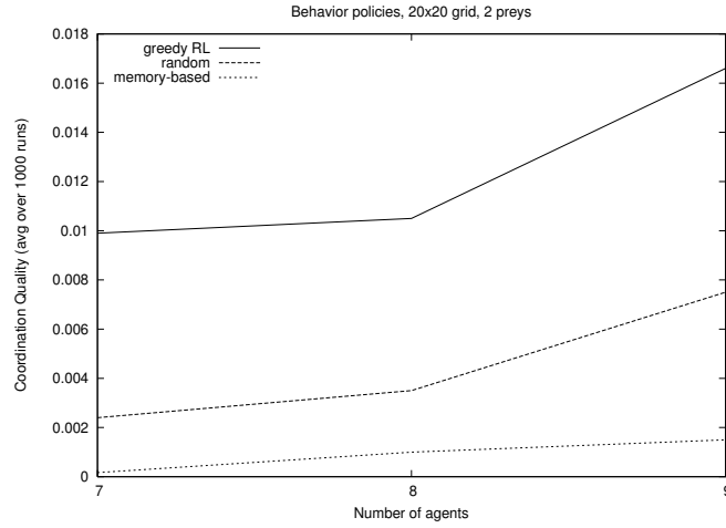
Fig. 1.6. Behavior policies
