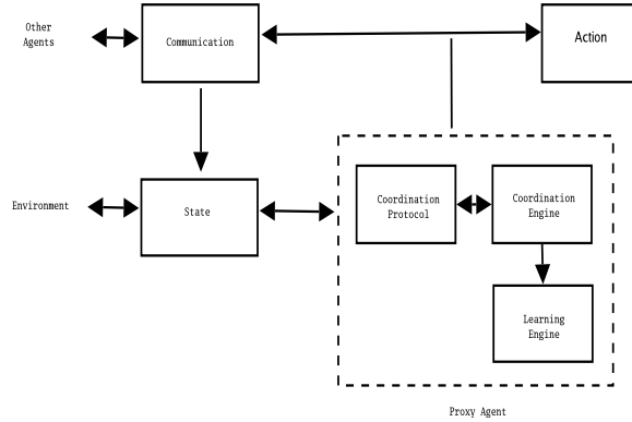
Fig. 1.1. Adaptive proxy agent architecture
