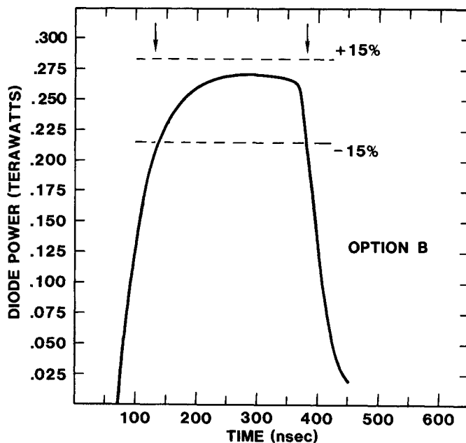
Fig. 6. Power delivered by the e-beam to anode.
