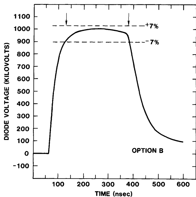
Fig. 5. Diode voltage waveform resulting from a Marx charge of 2.1 MV and an output switch closure of 1.07 \mu sec.
