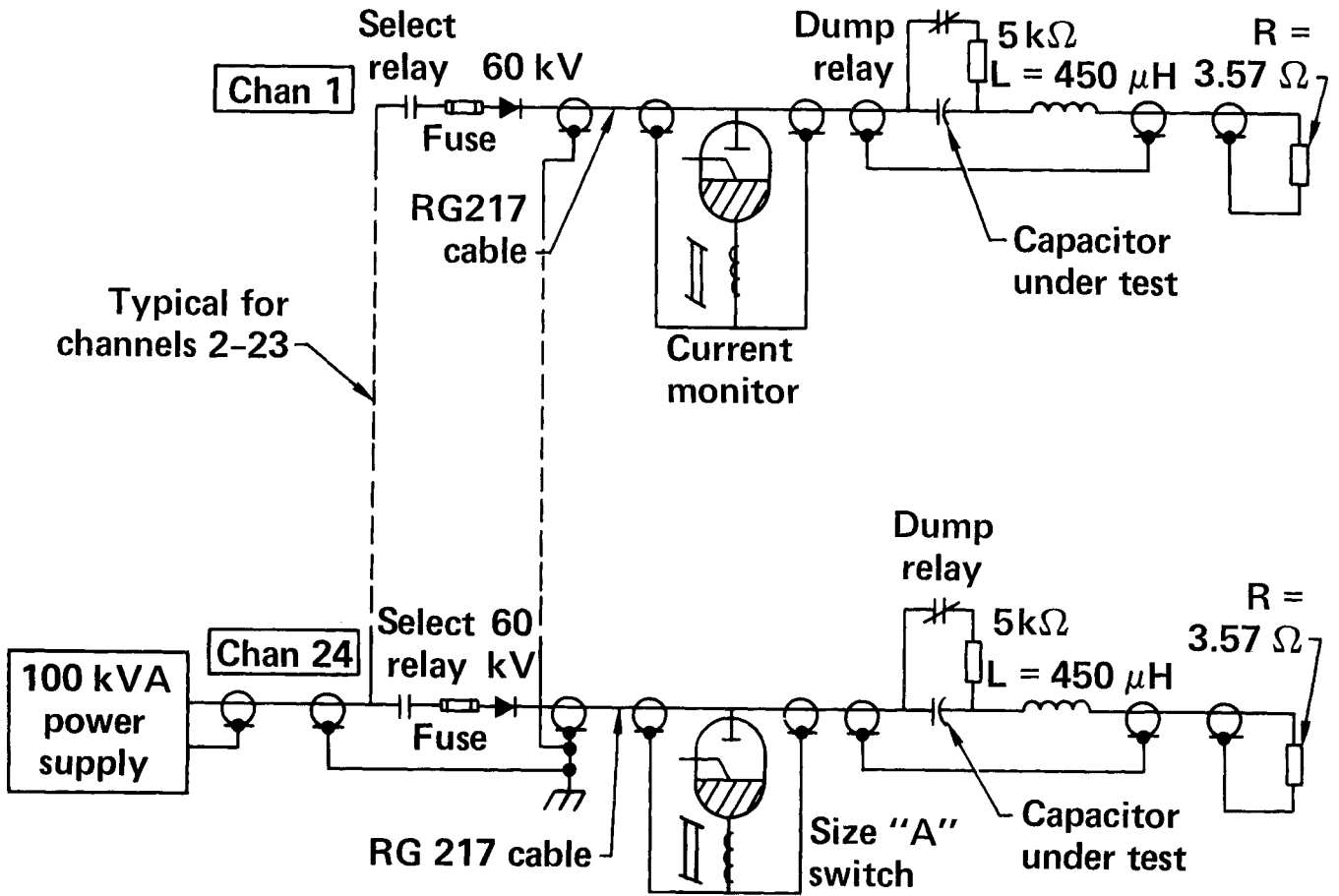
FIGURE 4 SCHEMATIC OF CAPACITOR TEST
