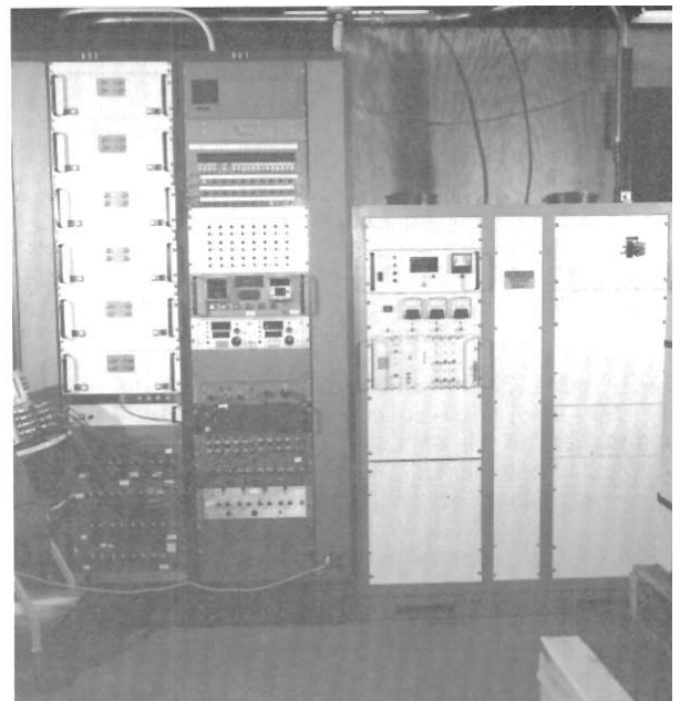
FIGURE 6 CONTROLS RACKS AND POWER SUPPLY
