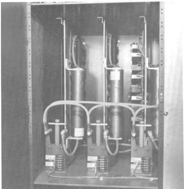
FIGURE 5 50 KV DIODE FANOUT
