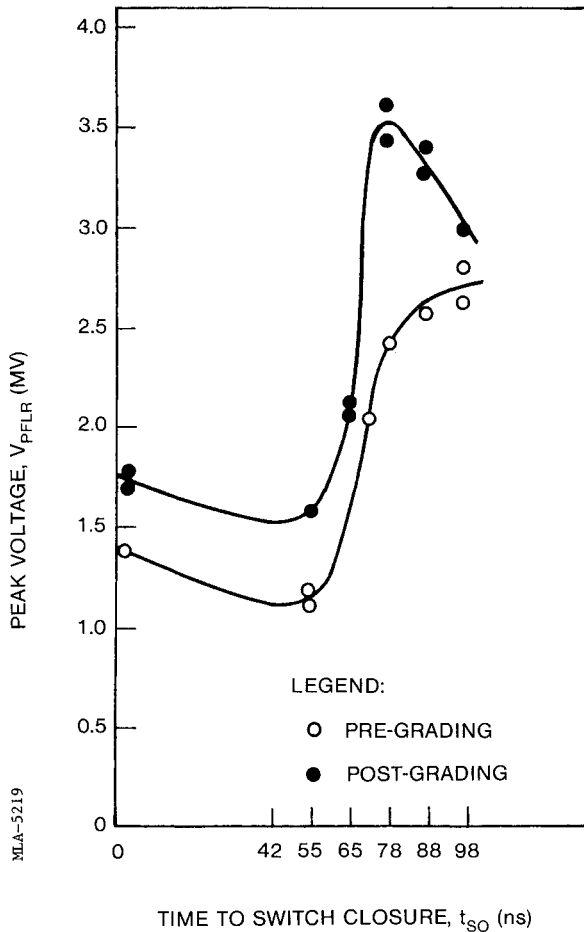
Figure 6. Variation of measured peak voltage at radial line probe position as a function of switch closure time, before and after grading (timing scan at 0.4 \hat{P}_o )
