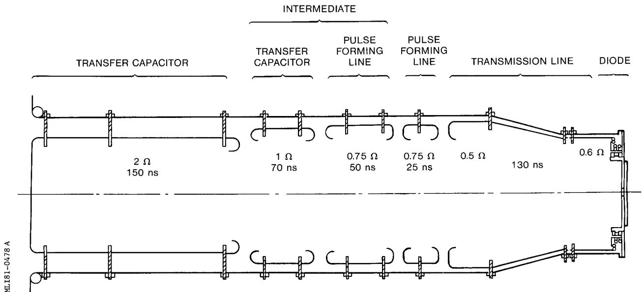
Figure 2. BLACKJACK 5 pulser, cross section
