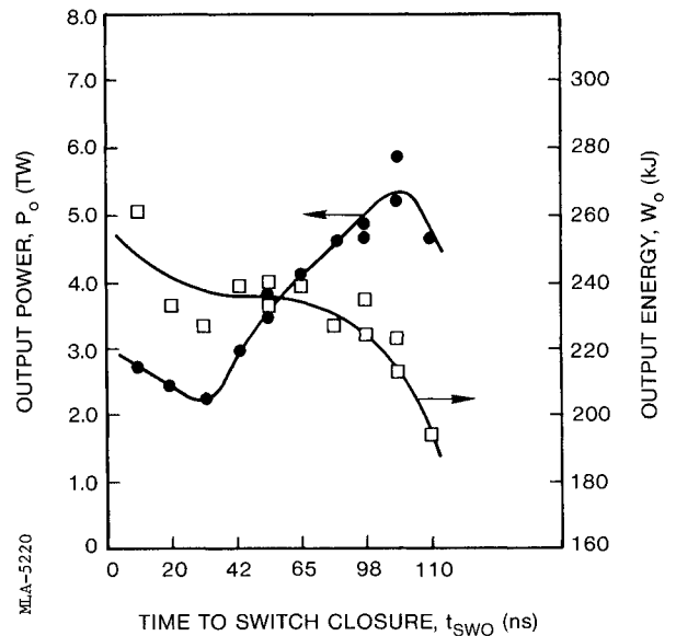
Figure 7. Variation of peak power and pulse energy with output switch closure time (timing scan at 0.4 \hat{P}_o )
