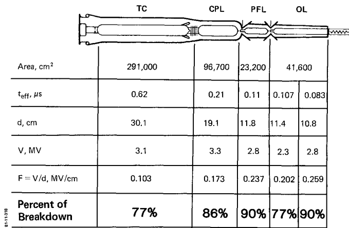
Figure 3. EAGLE waterline stresses at 4 TW. Voltage and average field maxima are given for shot 243.
