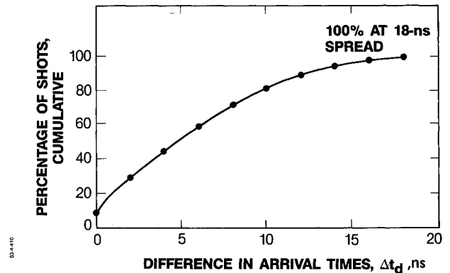
Figure 5. Double-EAGLE synchronism prediction. EAGLE shot-to-shot data is arranged in pairs to give Δt d , the arrival-time differences.
