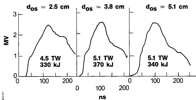
Figure 7. Output waveshape variability. The shape of voltage across the load is varied by changing PFL switch spacing. The shapes vary from double-bounce switching (7a) to conventional switching waveforms (7c).
