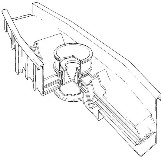
Figure 13. Artist's rendering of the Double-EAGLE coupler, which includes the transit time equalizer. The tube and vacuum feed region are at the center of the rendering.
