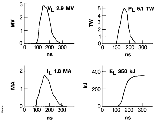
Figure 8. Output waveforms at 5.1 TW. Voltage, current, power, and energy for a maximum power shot on EAGLE are shown.
