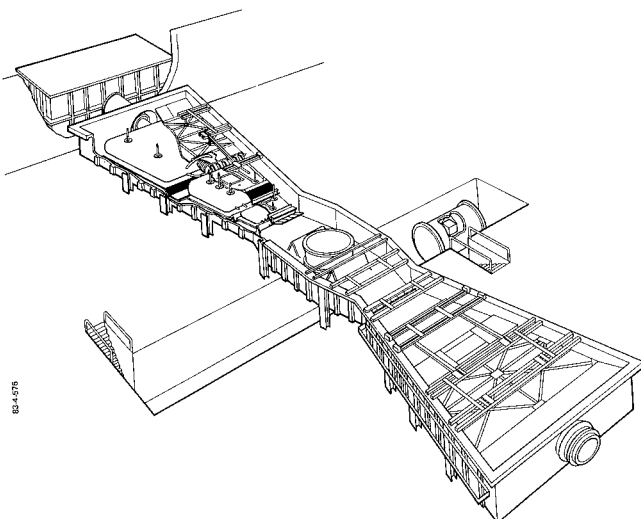
Figure 10. Artist's rendering of the Double-EAGLE generator.
