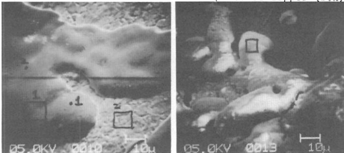
Figure 8 SEM micrograph of the middle region of a K-33 electrode used in air.
