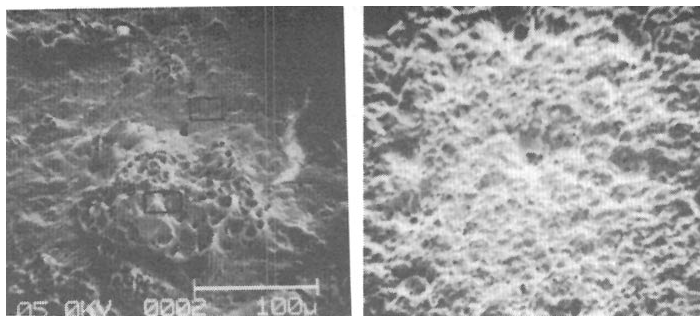
Figure 2 SEM micrograph of the inner region of a stainless steel electrode used in nitrogen.
