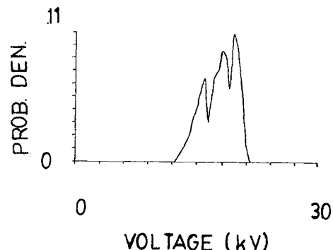
Figure 11 Self-breakdown voltage distribution for a stainless steel electrode in flowing air. (mean = 18 kV, standard deviation = 2 kV)
