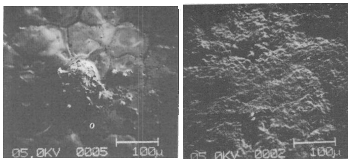
Figure 4 SEM micrograph of the inner region of a stainless steel electrode used in air.
