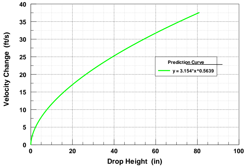
Figure 14. Prediction Curve for Velocity Change with AFD: Red Programmers
