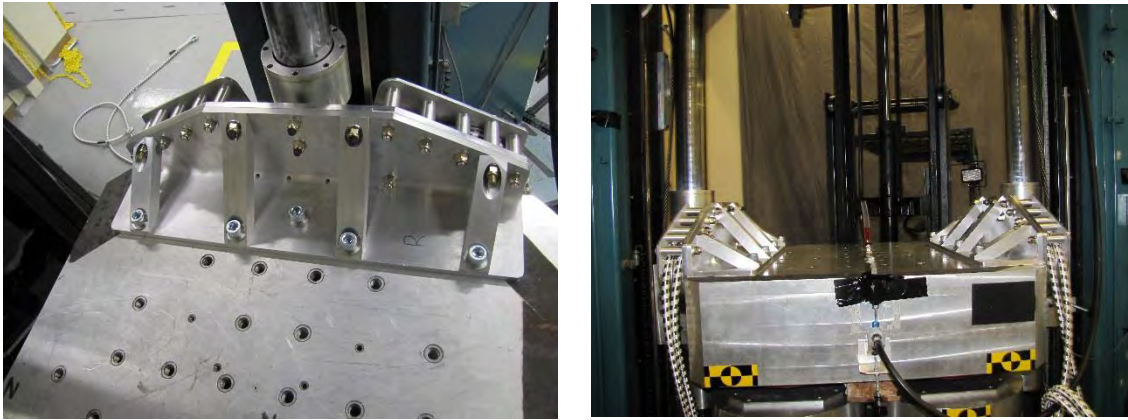
Figure 5. Top and Front View of VID Carriage Showing Location of AFD Guide Track
