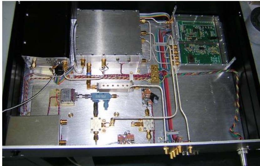
Figure 9. Picture of LO electronics.
