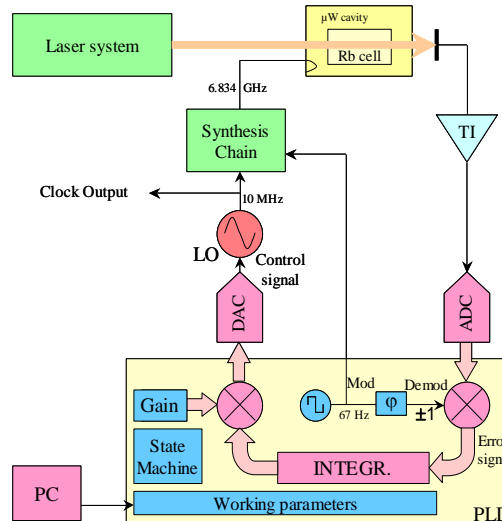
Figure 7. Block diagram of LO electronics.
