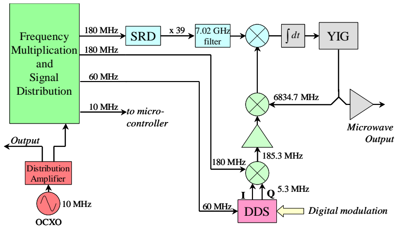
Figure 8. The block diagram of synthesis chain.
