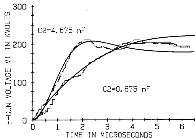
Figure 11. Comparison of Calculated and Experimental Voltage Variation.
