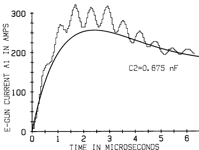
Figure 12. Comparison of Calculated and Experimental Current Variation.
