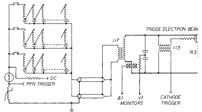
Figure 2. E-Gun Modulator Arrangement
