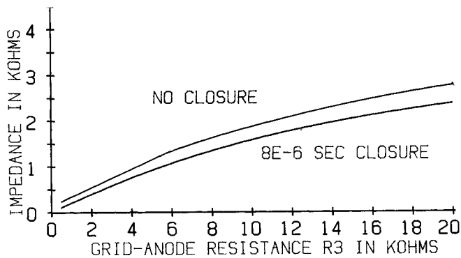
Figure 5. E-Gun Impedance vs Grid Resistance R3.
