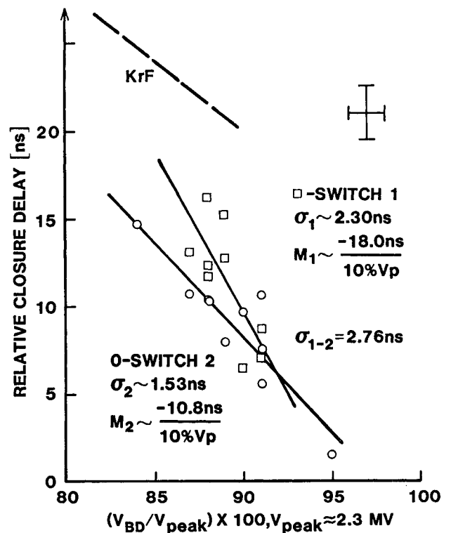
Figure 8. Double switch triggering results
