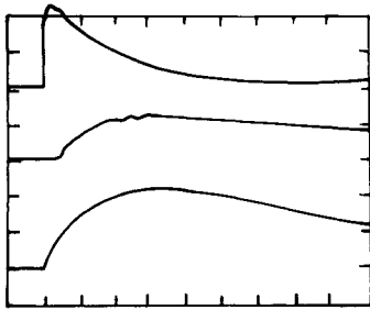
Fig. 7. Oscillograms from EMC test. Upper curve: applied current pulse, 10 kA/div; 10 ms/div. Middle curve: rotor speed 450 rpm/div; 10 ms/div. Lower curve: voltage across EMC 1 V/div; 10 ms/div.
