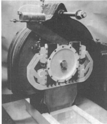
Fig. 5. Installation of EMC in dc magnet. (a) magnet half assembled. (b) fully assembled system.
