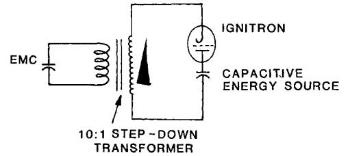
Fig. 6. Schematic of EMC test circuit.
