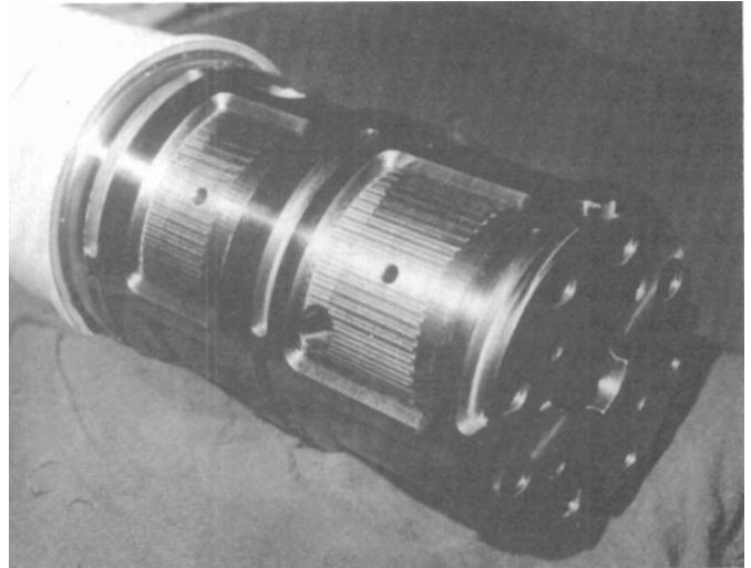
Fig. 8. Stationary-shaft bearing pockets
