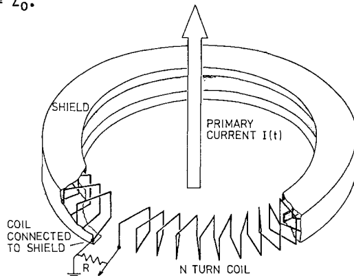
Fig 1a Geometry of the current probe
