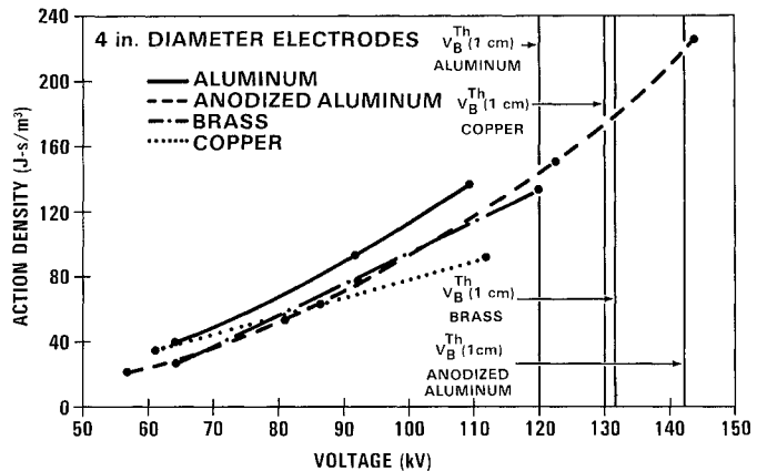
Figure 9. Action density as a function of applied voltage for various electrode materials. Note the threshold breakdown voltages (for a 1 cm gap) and the improvement of anodized aluminum over bead blasted aluminum.
