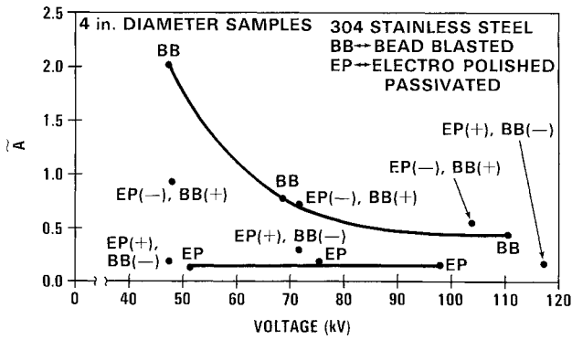
Figure 4. The normalized charge injection parameter, \tilde{A} , as a function of applied voltage for different coatings on 304 stainless steel.
