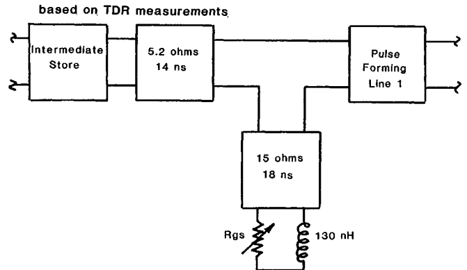
Figure 4. SCREAMER transmission line gas switch region model.
