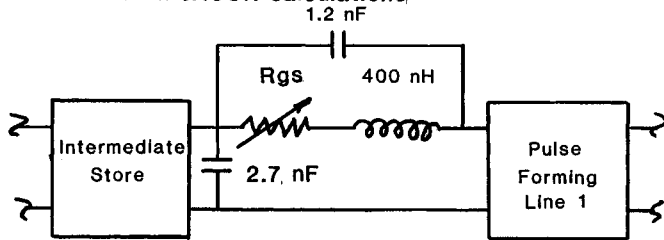
Figure 2. Original SCREAMER gas switch region model.
