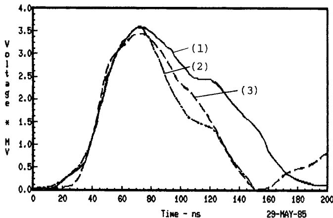
Figure 8. Lower transformer forward-going voltage: 1) SCREAMER model, 2) model with prepulse shield losses, and 3) measured Demon waveform.
