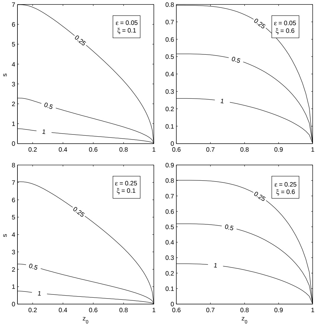
Fig. 7. Dependence of s(z_0, \xi, q^2) on the initial condition error z_0 for three different values of \sigma (0.25, 0.5, 1.0) and given values of q^2 ( =0.2 ) and \mu ( =1 ) using the Kaldor model with two different values of \epsilon (0.05, 0.25) and two different values of noise level \xi (0.1, 0.6). Note that the standard deviation of FTP is not sensitive to \sigma .
