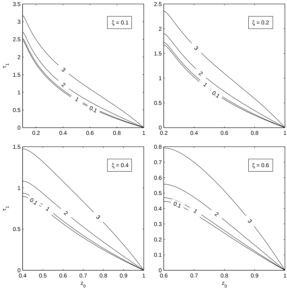
Fig. 4. Dependence of \tau_1(z_0, \xi, \varepsilon) on the initial condition error z_0 for four different values of \varepsilon (0.1, 1.0, 2.0, 3.0) and four different values of random noise \xi (0.1, 0.2, 0.4, 0.6) using the Kaldor model with given model parameters \sigma = 1.0 , q^2 = 0.2 , \mu = 1 .
