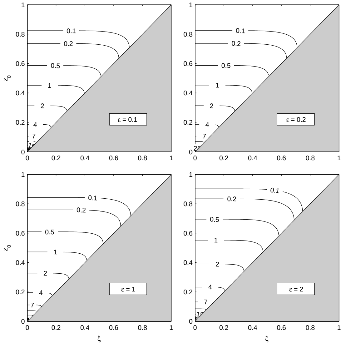
Fig. 3. Contour plots of \tau_2(z_0, \xi, \varepsilon) versus (z_0, \xi) for four different values of \varepsilon (0.1, 0.2, 1.0, 2.0) using the Kaldor model with given model parameters \sigma = 1.0 , q^2 = 0.2 , \mu = 1 . The contour plot covers the half domain due to z_0 \geq \xi .
