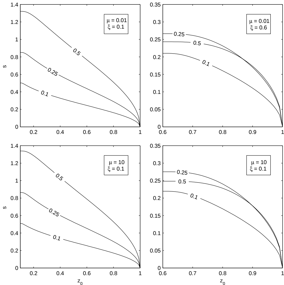
Fig. 9. Dependence of s(z_0, \xi, q^2) on the initial condition error z_0 for three different values of q^2 (0.1, 0.25, 0.5) and given parameters ( \sigma = 1.0 , \varepsilon = 0.2 ) using the Kaldor model with two different values of the adjustment coefficient \mu (0.01, 10) and two different values of noise level \xi (0.1, 0.6). Note that the mean FTP is not sensitive to varying \mu .
