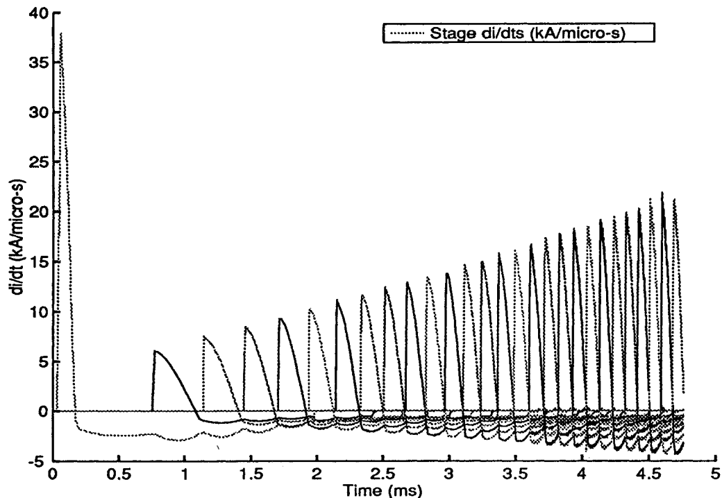
Figure 4. Stage di/dt's
