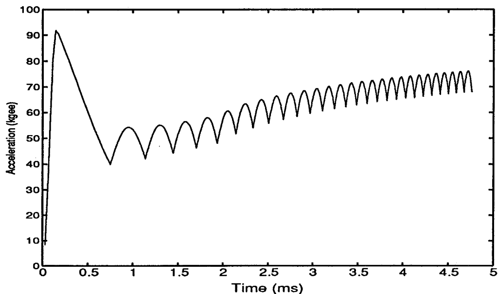
Figure 3. Projectile Acceleration
