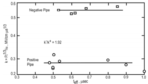
Figure 5(a). Oil polarity effect in 4-5 MV 10 4 cm 2 Aurora tests.
