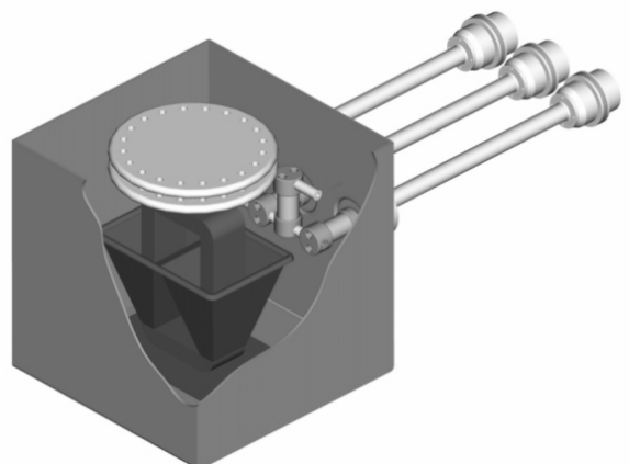
Figure 6. Electra oil test configuration.
