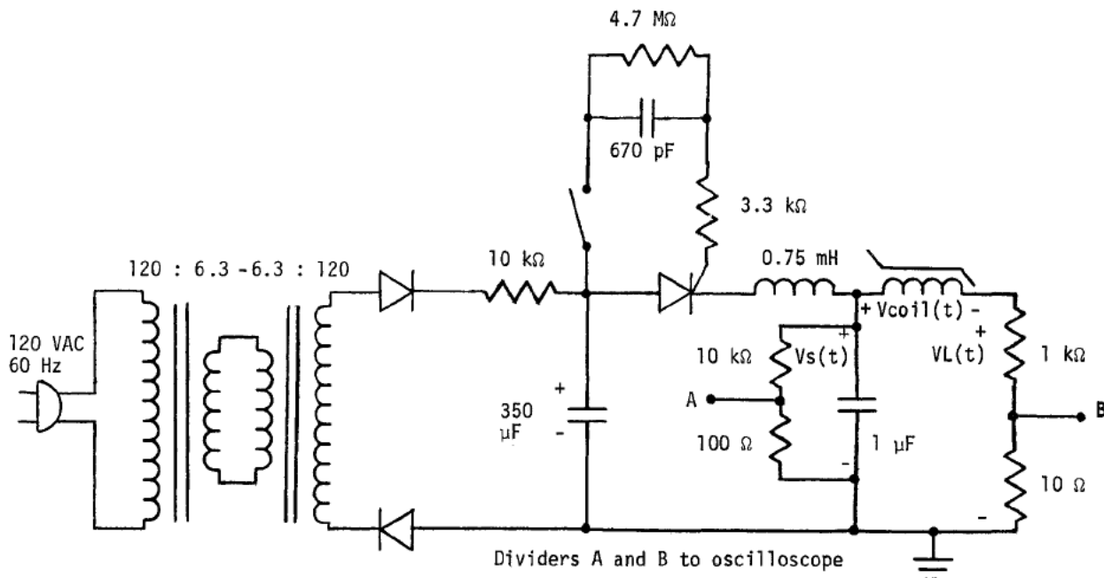
Figure II-1. Magnetic Switch Circuit.
