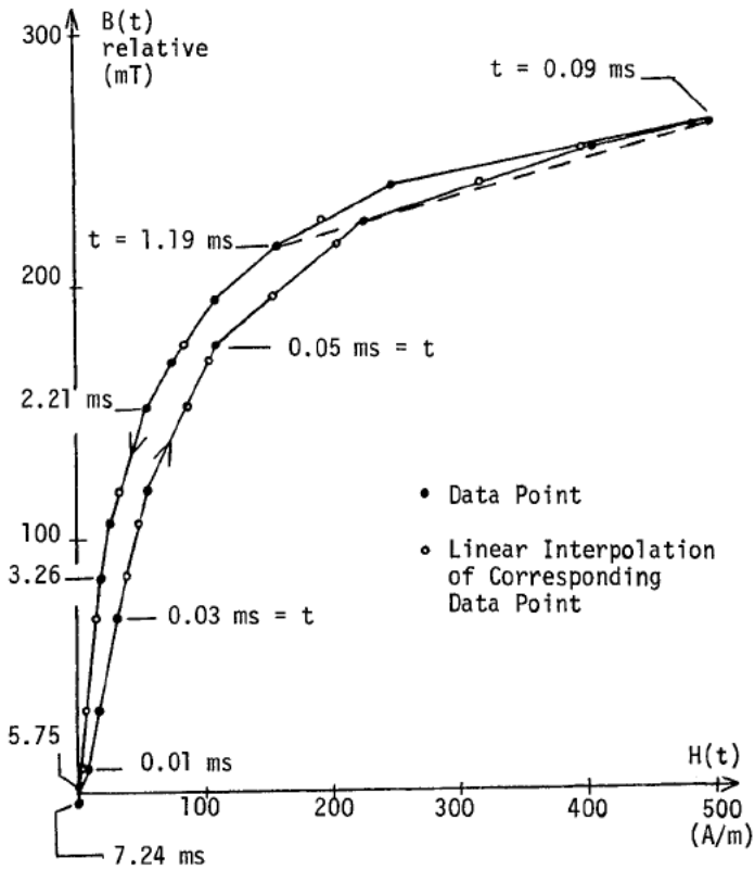
Figure IV-2. Energy lost to hysteresis.
