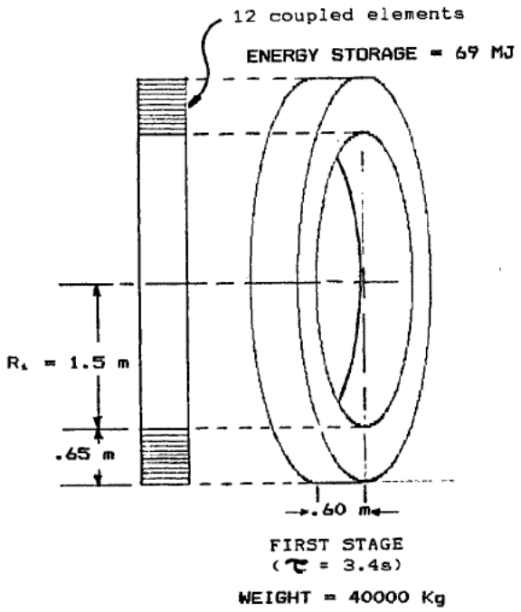
Figure 4. Geometry of the 11 step Meatgrinder.
