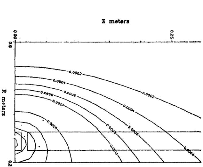
Figure 3. Representative field plot used in the calculations of the self and mutual inductances for the coil design.
