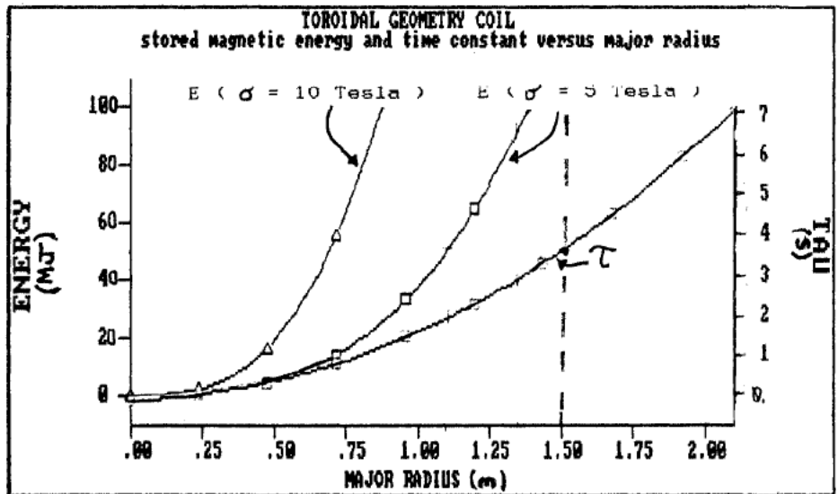
Figure 1. The variation of inductor time constant and stored magnetic energy as a function of major radius.
