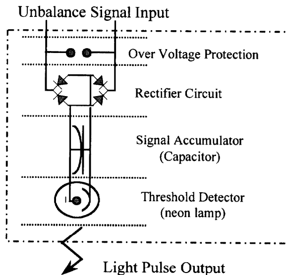
Figure 7. Typical threshold detector (Relaxation Oscillator).
