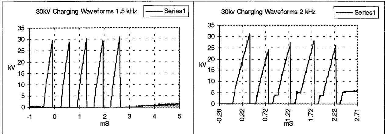
Figure 7 Charging Waveforms at 1.5 kHz Rep-Rate. Figure 8. Charging Waveforms at 2 kHz Rep-Rate.
