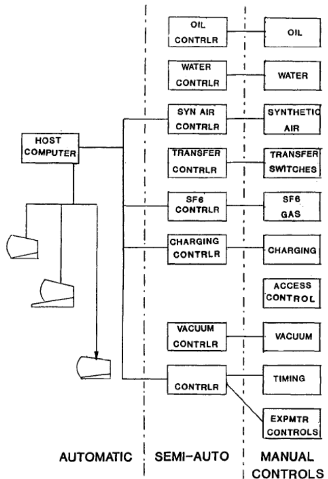
Figure 1. Hardware Configuration
