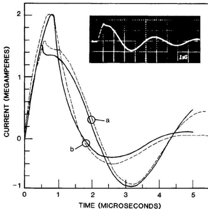
Fig. 4. Computed (solid) and experimental (dashed) electrical current for the LLNL electric gun aluminum foils ( V=90 kV, C=15.1 \mu\text{F} , L=25 nH, R=1 m \Omega , \delta=50.8 \mu\text{m} , l=\omega , tamper \rho\delta=0.427 kg/m ^3 ): (a) \omega=5.08 cm; (b) \omega=10.2 cm. The inset shows the actual oscilloscope trace for (a).
