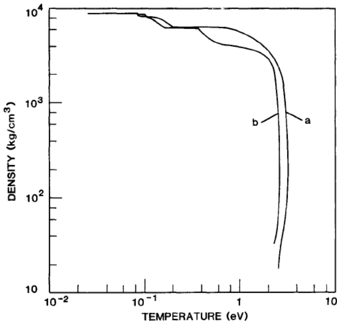
Fig. 10. Density-temperature trajectories for the foils of Fig. 7.
