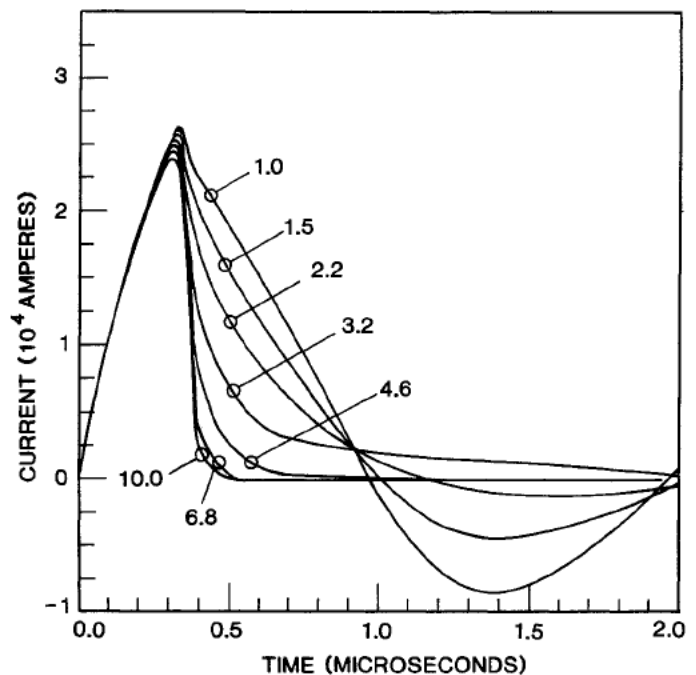
Fig. 11. Predicted electrical current for the parameters of Fig. 7a and foil length (mm) as indicated.
