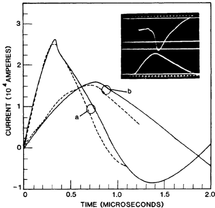
Fig. 7. Computed (solid) and experimental (dashed) electrical current for the Los Alamos slapper test facility copper foils ( V=5 kV, C=2 \mu F, R=30 \mu \Omega , \delta=20 \mu m, l=1 mm, \omega=1.12 mm, temper \rho\delta=0.291 kg/m 2 ): (a) L=45 nH; (b) L=160 nH. The inset shows the actual voltage and current oscilloscope traces for (a).
