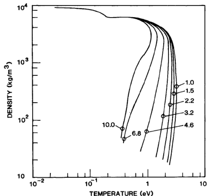
Fig. 12. Density-temperature trajectories for the foils of Fig. 11.
