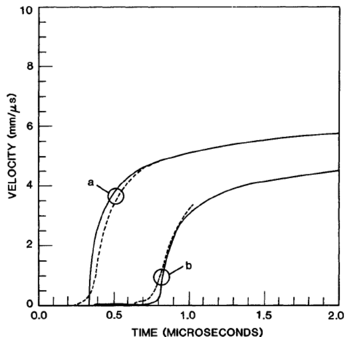
Fig. 9. Computed (solid) and experimental (dashed) expansion velocity for the foils of Fig. 7.
