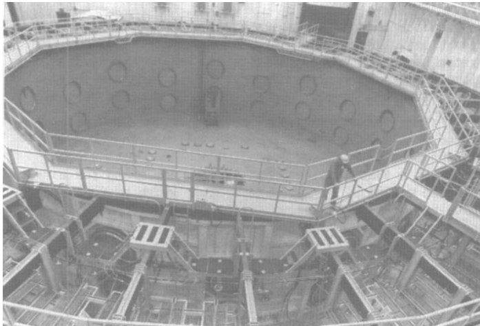
Figure 2. Accelerator tank.
