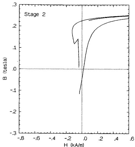
Fig. 4. Hysteresis loop of second magnetic switch.
