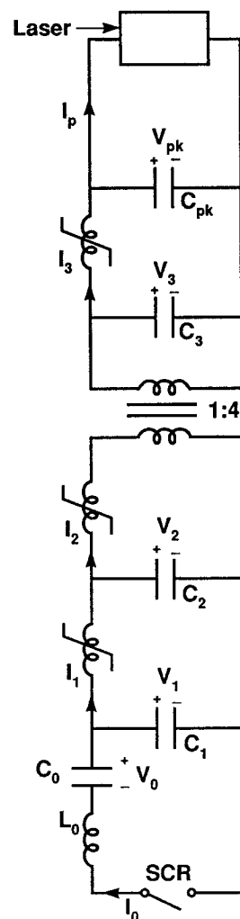
Fig. 1. Schematic modulator circuit. The reset circuit is not shown
