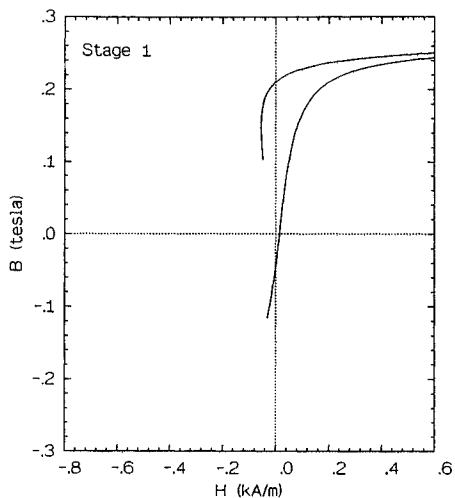
Fig. 3. Hysteresis loop of first magnetic switch.
