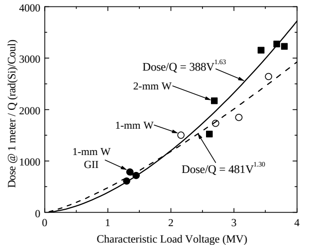
Figure 3. Scaling of the measured dose, normalized to charge, with the characteristic voltage. The squares and open circles are ASTERIX measurements for 2-mm and 1-mm diam anodes, respectively. The filled circles are Gamble II measurements.
