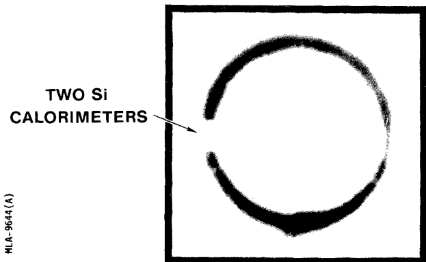
Figure 6. X-ray image of the BLACKJACK 5 25 cm dia tantalum converter showing the location of the silicon calorimeters.
