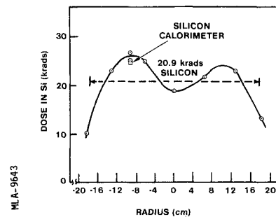
Figure 10. The horizontal, radial dose profile as measured by several TLD-200s (CaF 2 :Dy) and a silicon calorimeter yielded an area weighted mean dose of 20.9 krads-Si over 1000 cm 2 .
